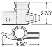
Lower Lock Rod Cam
