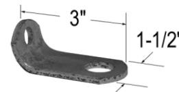
1. FRUDCE8363-1 Latch
