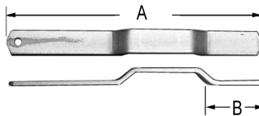
1. FRUDCE8361-1 Door handle A = 16-11/16" B = 6-5/16"
