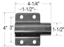
1. FRUDCF3527-1 Guide back plate
