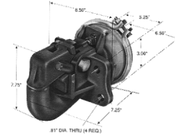
Less plunger, air cylinder, & bracket
